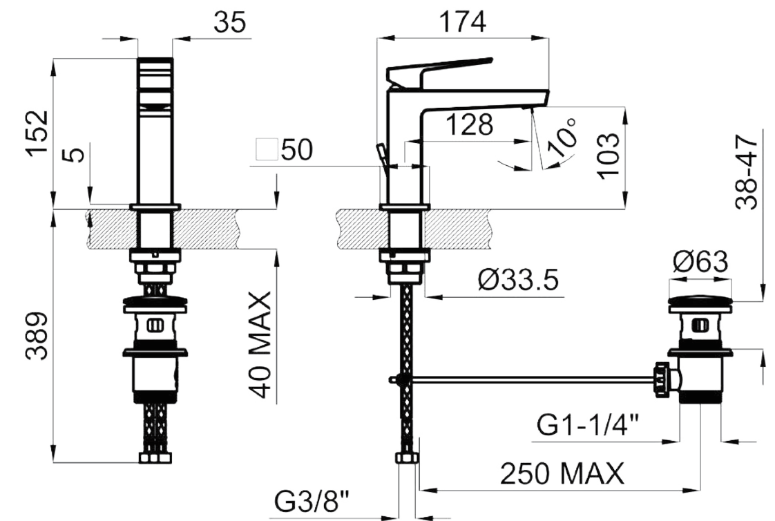
Technical Drawing 規格表(mm)
